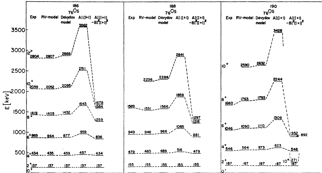
FIG. 1. The energies of the ground-state bands of Os 186 , Os 188 , and Os 190 . [Exp—experimental energies of Lark, Gugelot, and Morinaga (Ref. 12), supplemented by the data of Refs. 1–11; RV model and Davydov models (see text); I(I+1) is the adiabatic Bohr-Mottelson model; and A \cdot I(I+1) - BI^2(I+1)^2 is the Bohr-Mottelson model with empirical rotation vibration corrections.]
